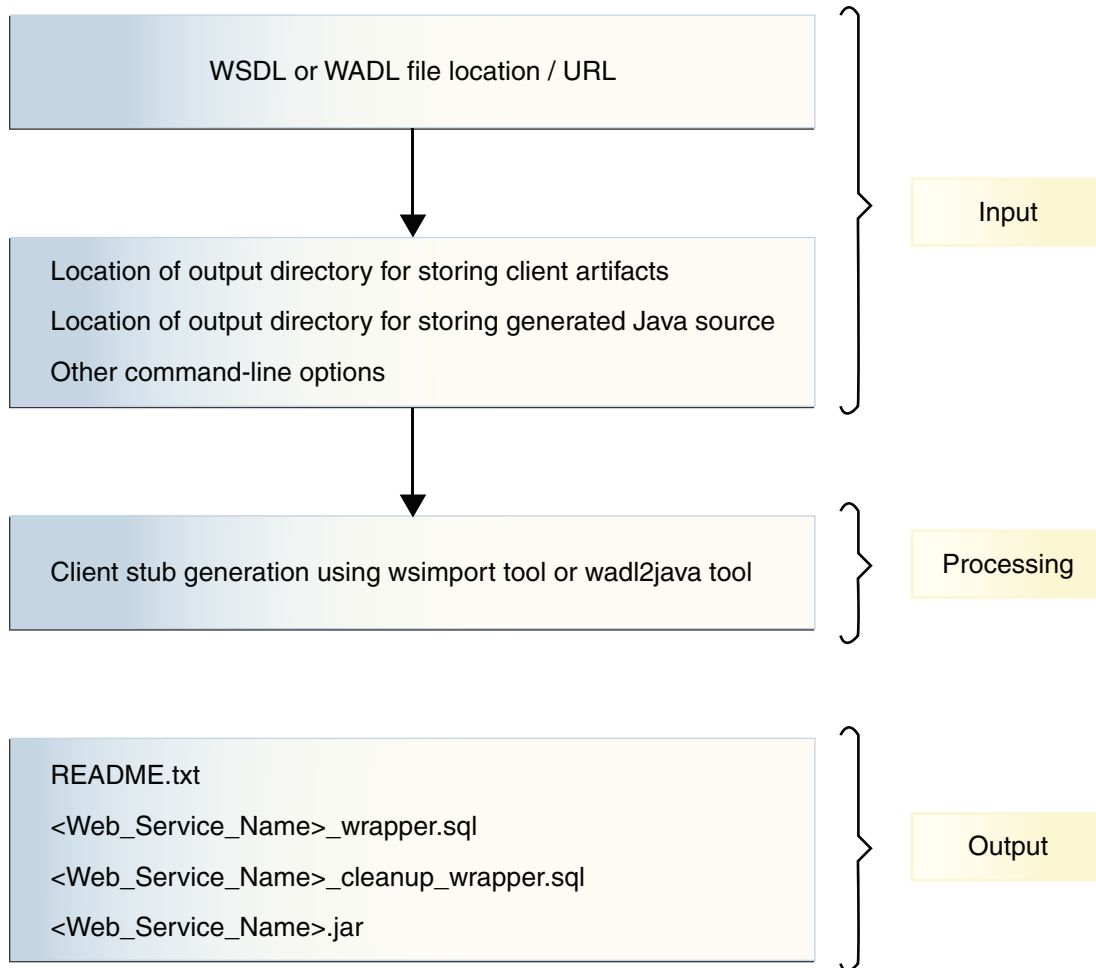
Figure 14-1 Oracle JVM Web Services Call-Out Utility Architecture
