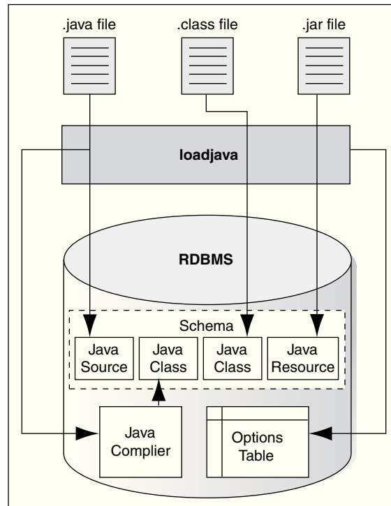
Figure 2-2 Loading Java into Oracle Database
